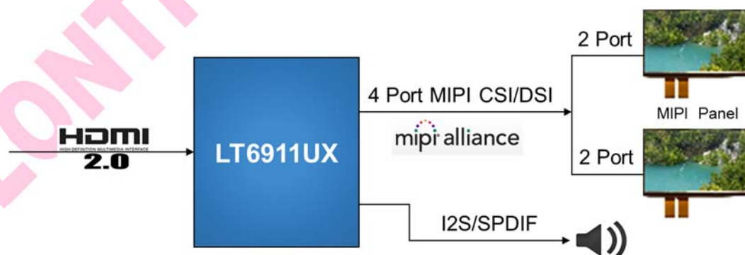
Figure1. Application Diagram
