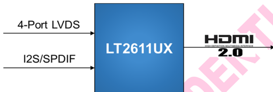
Figure1. Application Diagram
