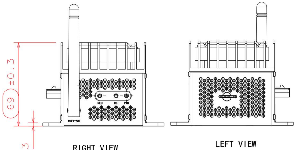
RIGHT VIEW
