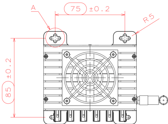
DOWN VIEW
