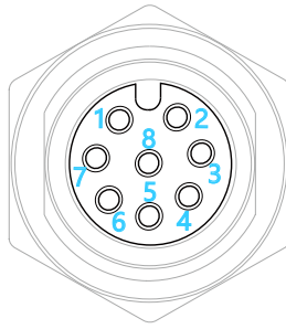
Figure 2 Pinout of the Connector
