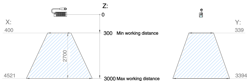
Figure 1 FOV (unit: mm)
