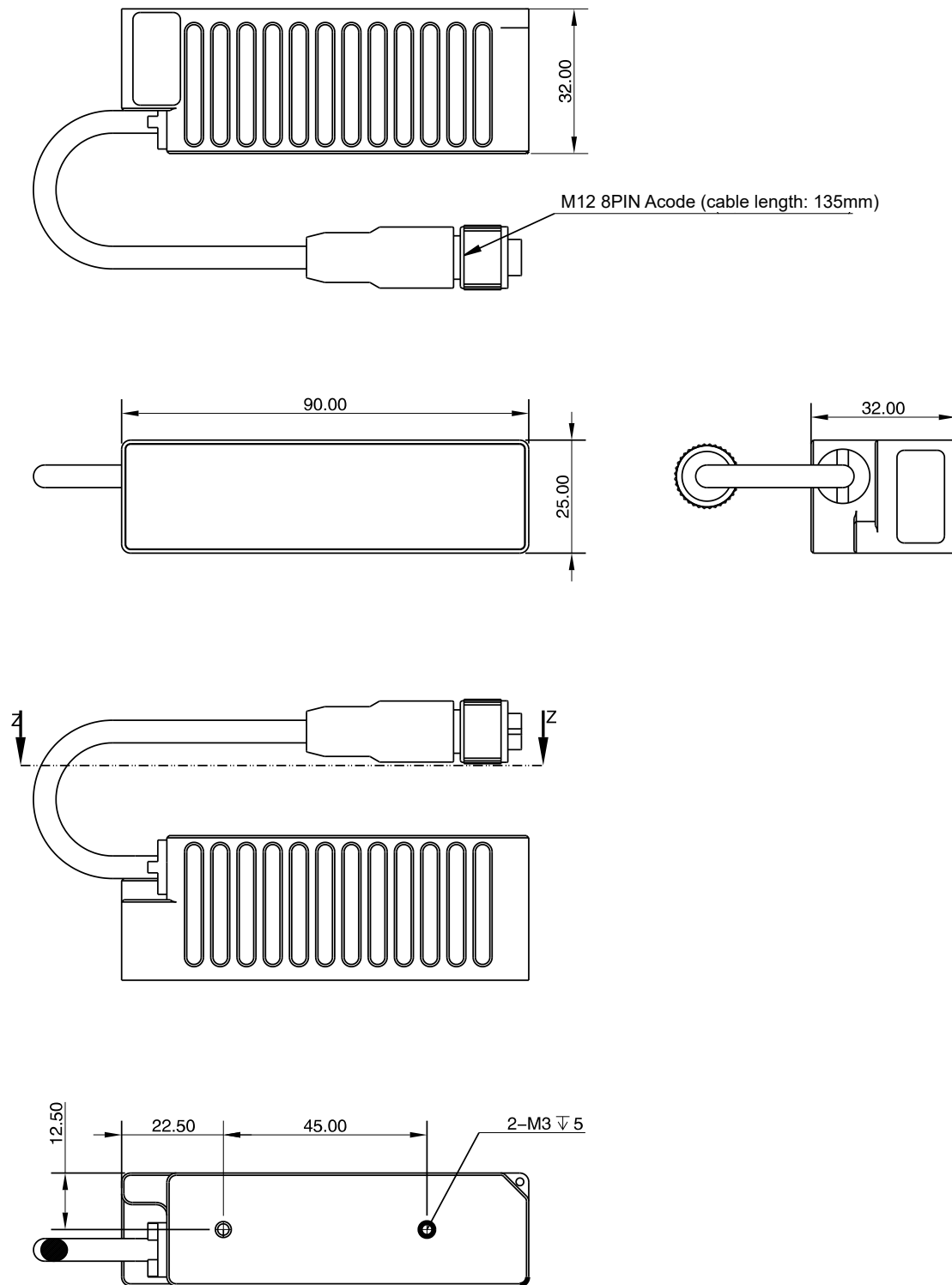
Z-Z Figure 3 GM465-E1 Mechanical Dimensions (unit: mm)
